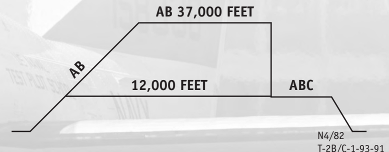
Figure 10-1. Checkflight Profile
